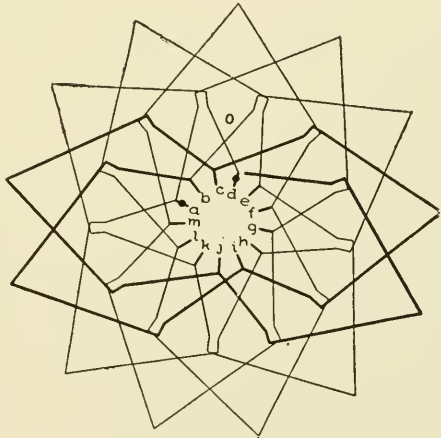
Fig. 140. Diagram Showing the Effect of Open-Circuited Coil Causing Sparking at the Commutator
